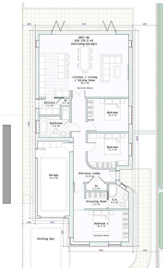
Proposed Ground Floor Plan (Scale 1:50 @ A1 / 1:100 @ A2)
